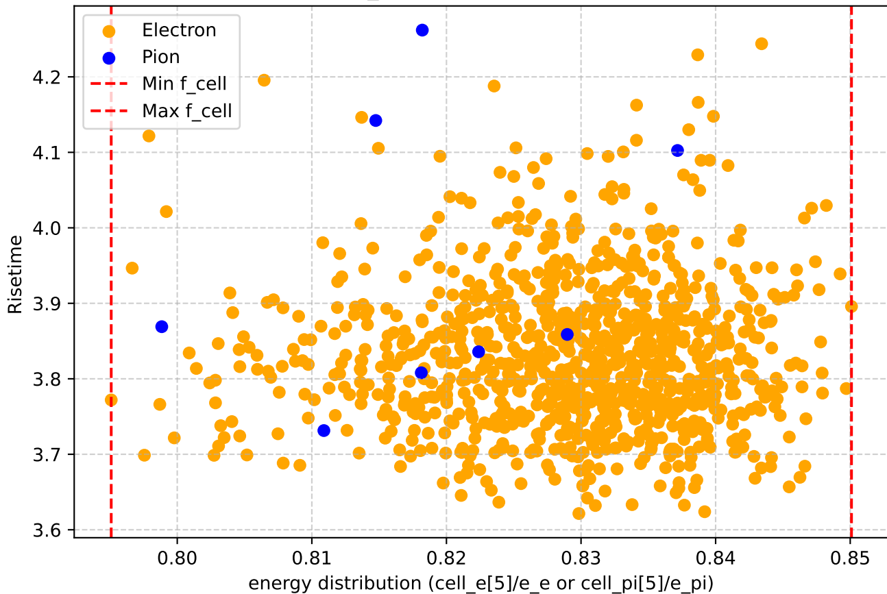
Scatter plot of f_{\text{cell}} vs risetime for energy 80.0GeV
